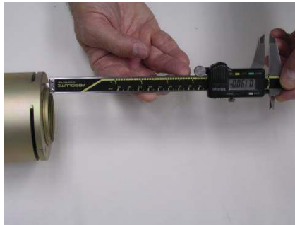
Picture 6P – Use of Drop Gage to measure stick-out
