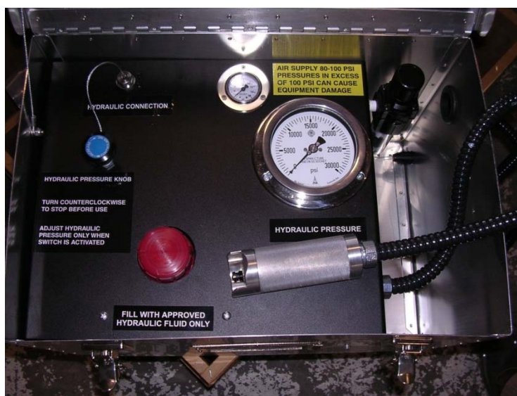
Sample Picture of AP-0532 Hydraulic Pump with hydraulic connection plugged for testing
