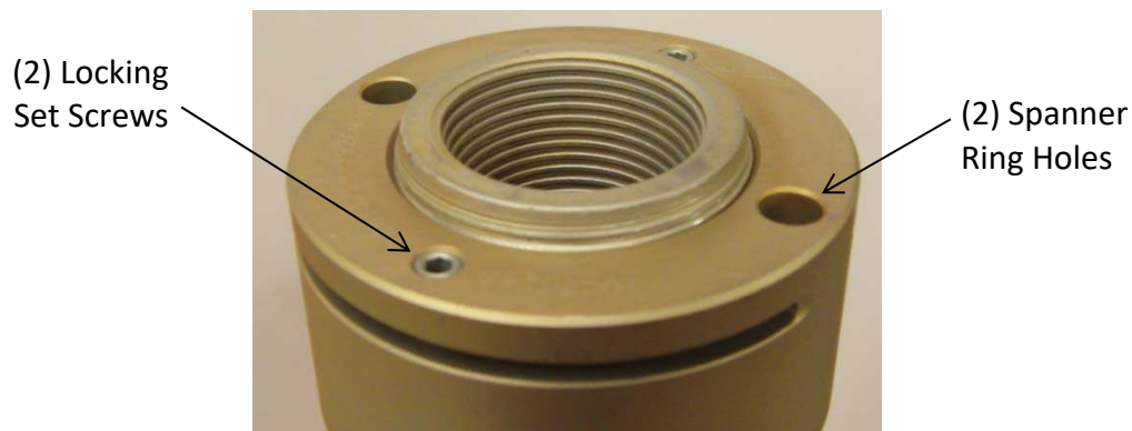
Figure 5A - Riverhawk Locknut
