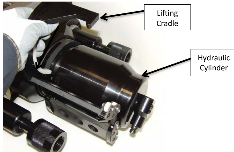
Figure 8D – Remove lift cradle from assembly
