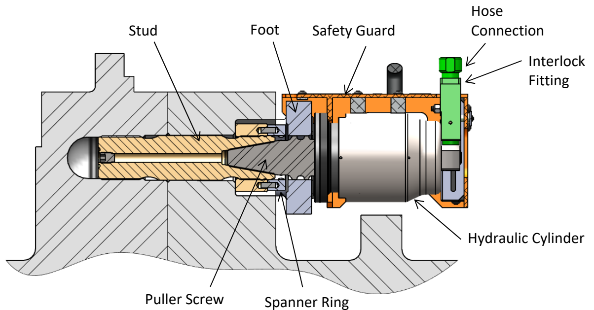
Figure 8F – Cutaway view of Hydraulic Tensioner HT-5298
