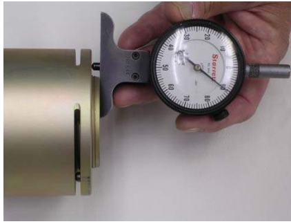
Figure 6B – Use of drop gage to measure stick-out
