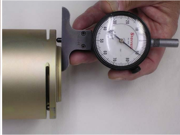
Drop Gage
