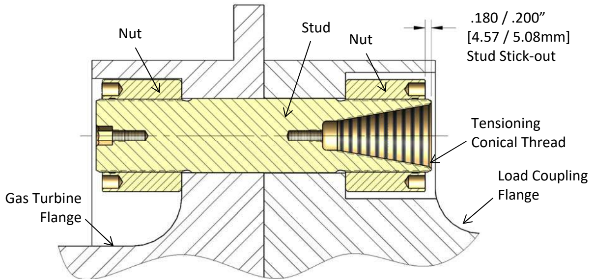
Figure 1 – Cutaway View of Turbine Flange and Coupling Flange Bolted Joint
