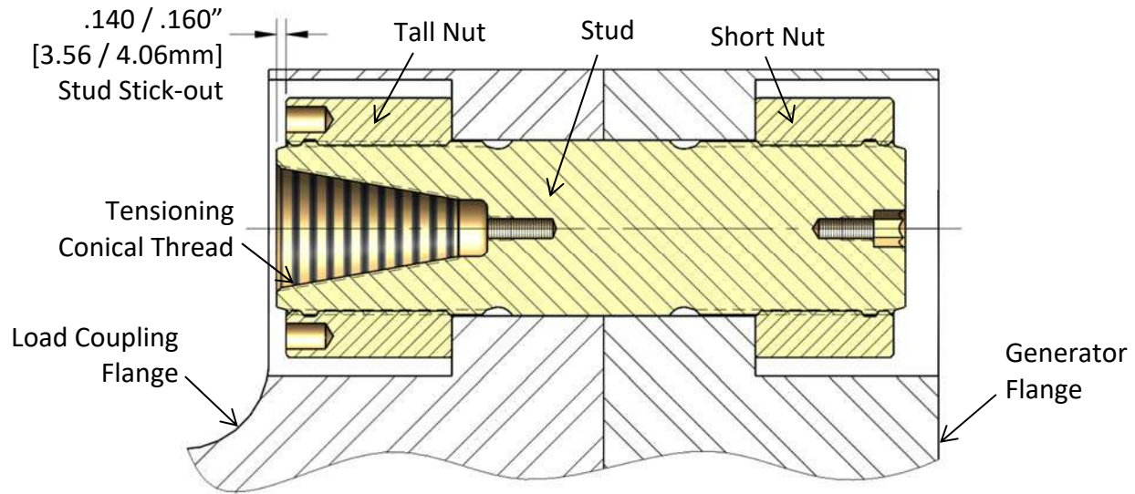
Figure 2 – Cutaway View of Generator Flange and Coupling Flange Bolted Joint
