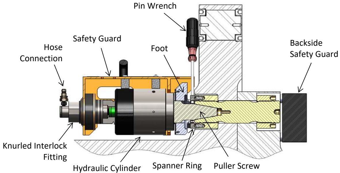
Figure 8D – Cutaway view of Hydraulic Tensioner HT-6019 (generator end only)
