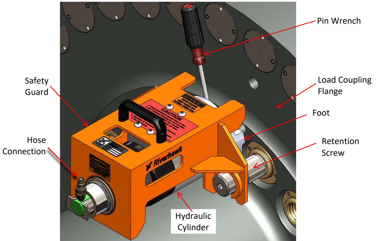
Picture 8C – Features of the Hydraulic Tensioner HT-6019 (generator end only)
