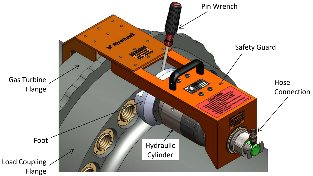
Picture 8A – Features of the Hydraulic Tensioner HT-6282 (turbine end only)
