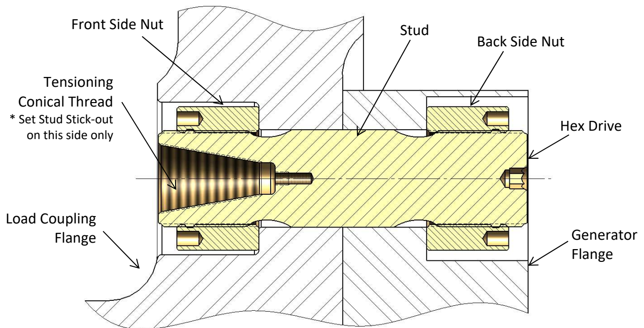
Figure 6B – Cross-section View of Load Coupling to Generator Bolted Flange Connection
