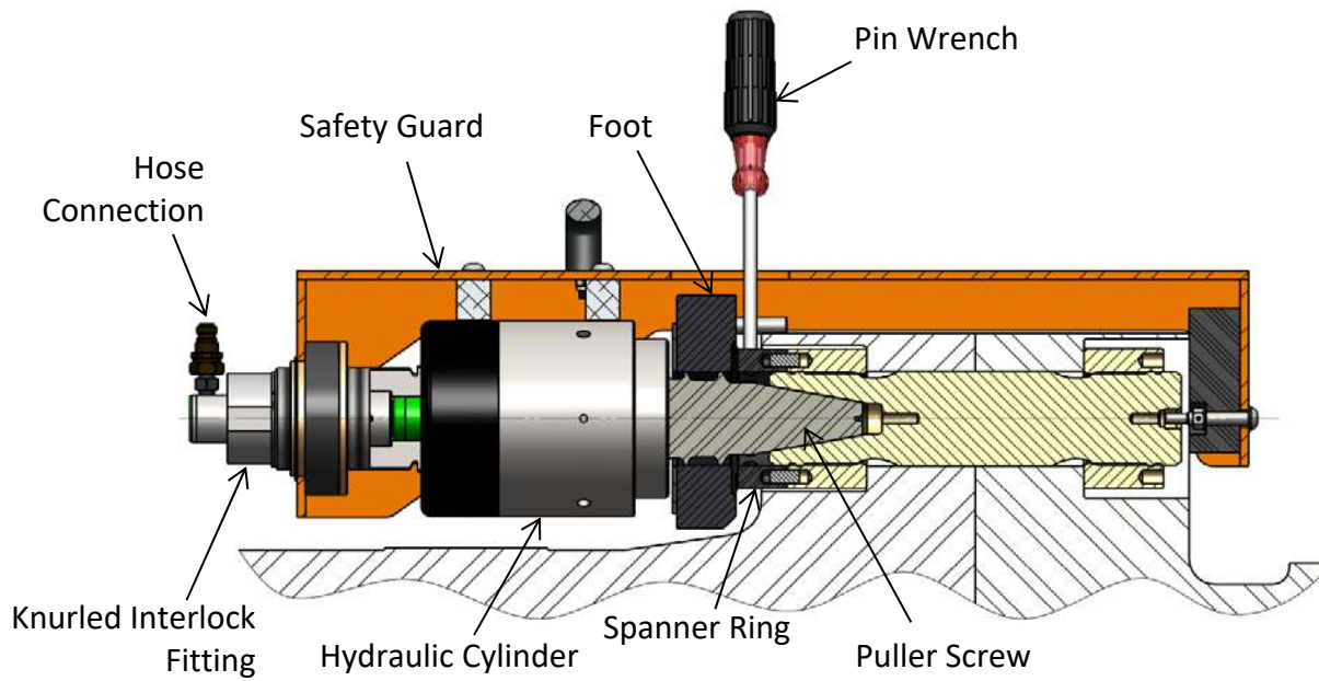
Figure 8D – Cutaway view of Hydraulic Tensioner HT-6525
