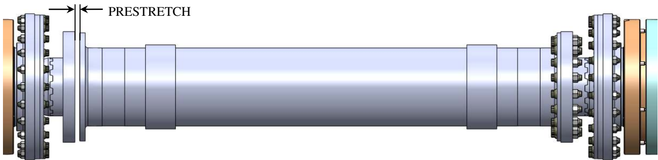
Figure 14 – Prestretch Gap Check at Final Bolted Joint
