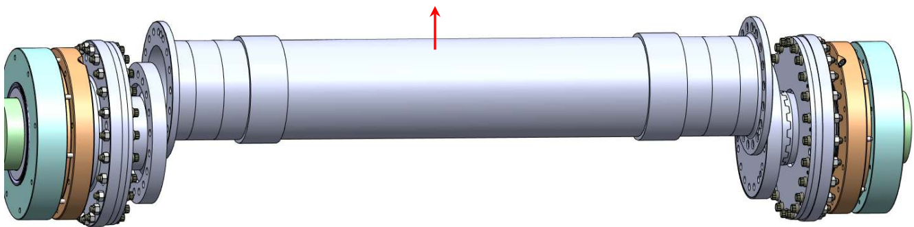
Figure 17 – Center Tube Removal
