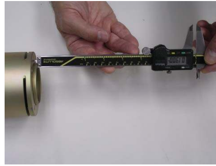
Picture 6K – Use of Calipers to measure stick-out
