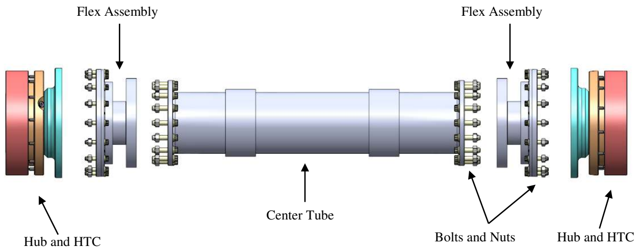
Figure 1 – Components
