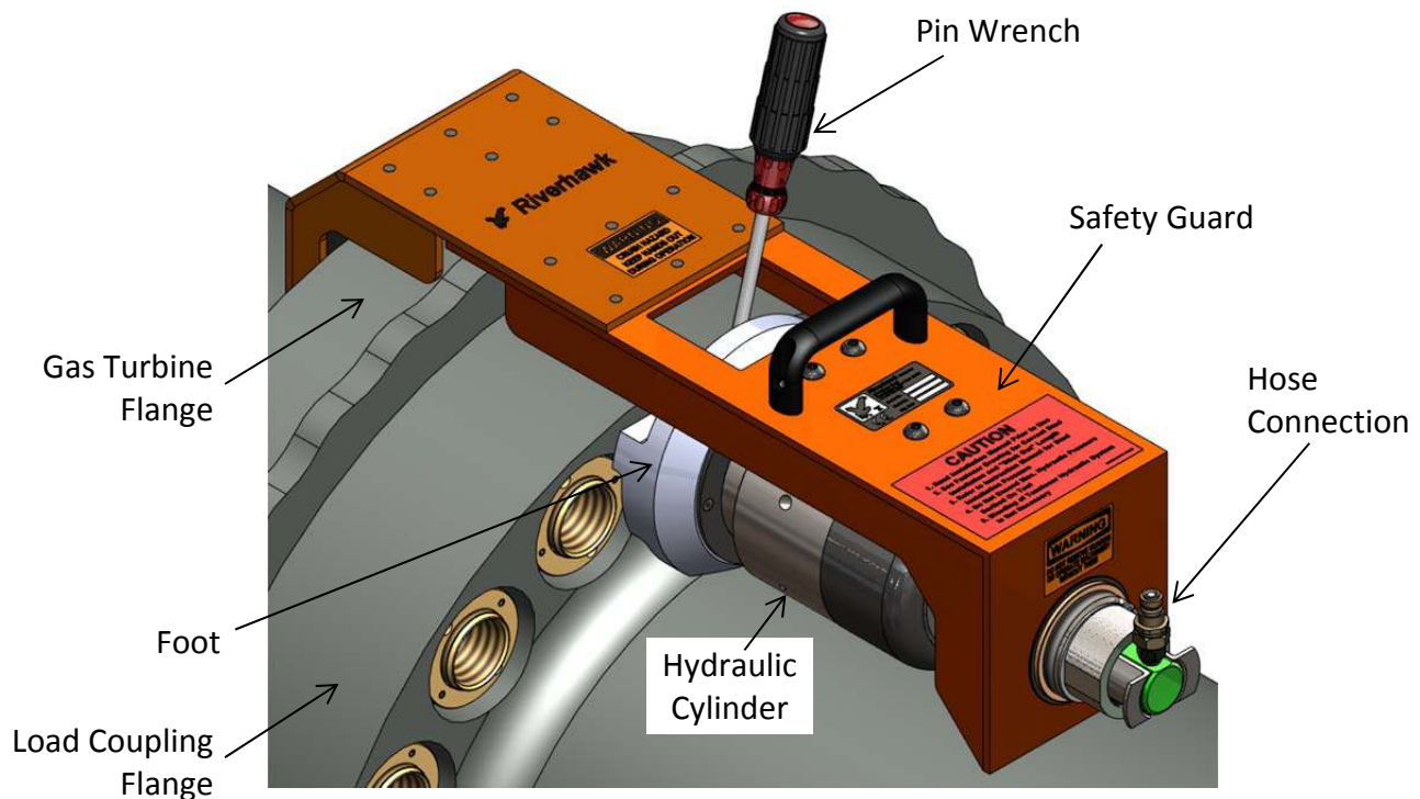
Picture 8A – Features of the Hydraulic Tensioner HT-6282 (turbine end only)
