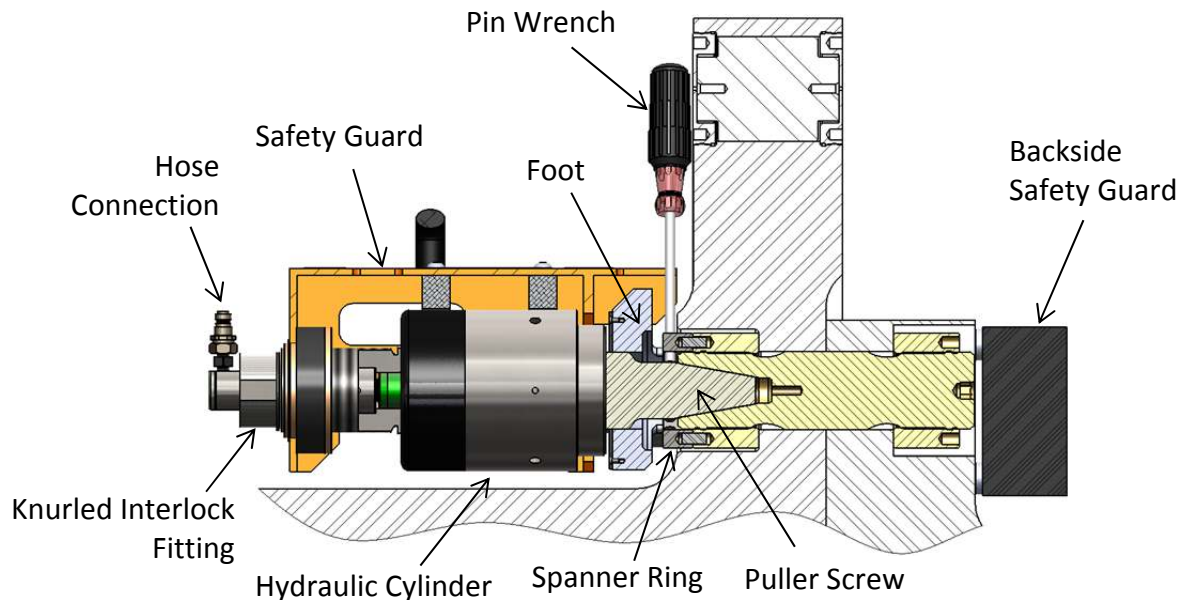
Figure 8D – Cutaway view of Hydraulic Tensioner HT-6019 (generator end only)
